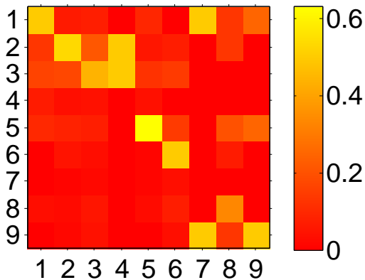
Figure 1: Confusion matrix of the prediction results. Rows represent the actual occupational class (C 1–9) and columns the predicted class.
